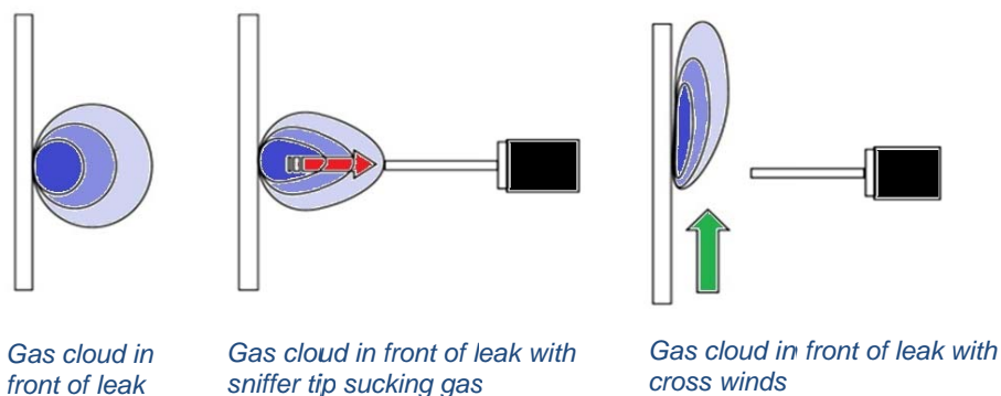
Fig. 5: Gas cloud in front of leak
