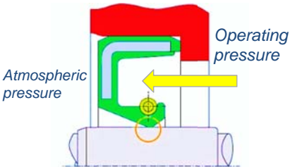
Fig. 4: Radial shaft seal
